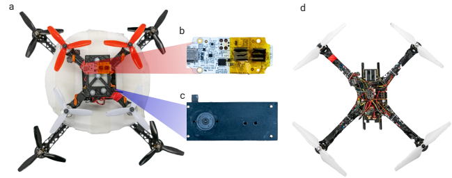
Figure 6. (a) Smaller quadrotor on the bigger quadrotor used for landing experiments (Sec. IV-A), (b) Gutted Coral USB Accelerator with custom heat sink used to run the neural networks, (c) Samsung Gen 3 DVS sensor used for experiments, (d) Bigger quadrotor used in the following experiments (Sec. IV-B).
